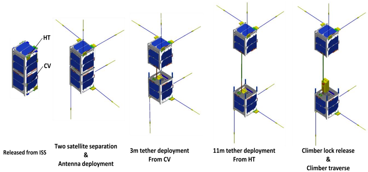
Fig.2- CAD MODEL
